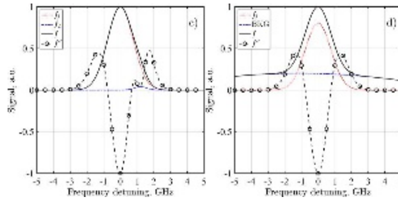
FIG. 1. Illustration of derivative spectroscopy. (a) Single Maxwellian VDF signal (solid black line) and its first ( f' , dashed line with crosses) and second ( f'' , dashed line with circles) derivatives. (b) Bi-Maxwellian VDF signal (dotted red and dashed blue lines) with nonzero most probable velocities and its second derivative f'' (dashed line with circles). (c) Bi-Maxwellian VDF signal with a bulk distribution (dotted red) and a smaller faster group (dashed blue) and its second derivative f'' (dashed line with circles). (d) Single Maxwellian VDF (solid black line) signal with a nonlinear (sinusoidal) background (BKG, dashed blue line) and its second derivative f'' (dashed line with circles). Distributions on each subplot are normalized to the maximum of the total distribution (solid black line). Signals and their derivatives were normalized to the maximum absolute value of each curve.
