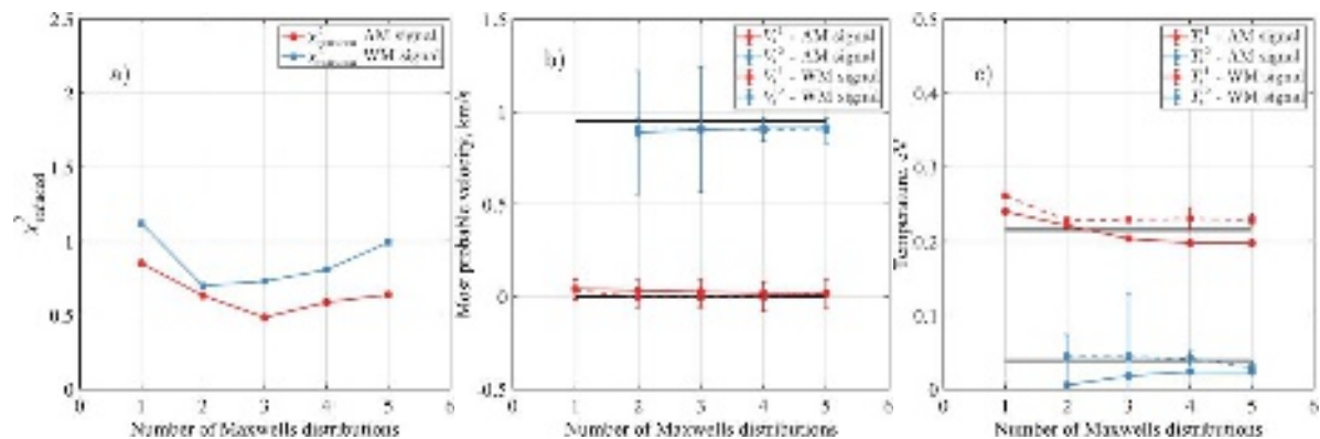
FIG. 5. Fitting results of modeled AM and WM signals with varying number of fitted distributions ( N = 1 to 5). (a) \chi_{red}^2 for AM (red) and WM (blue) signals. (b) Most probable velocity for bulk ( V_i^1 , red solid for AM and blue solid for WM signals) and fast ( V_i^2 , red dashed for AM and blue dashed for WM signals); black lines show “ground truth” values. (c) Same as (b) but for temperatures.
