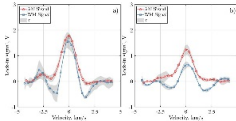
FIG. 9. Experimentally obtained AM signals or IVDF profiles (red, circles) and their WM signals, or IVDF second derivatives (blue, squares) for two locations (central and middle). The shaded area represents the standard deviation of three measurements.
