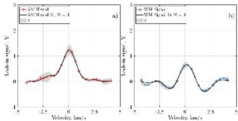
FIG. 13. The best fits of the a) AM signal and b) WM signal at the middle location. N shows the number of Maxwellian distribution.
