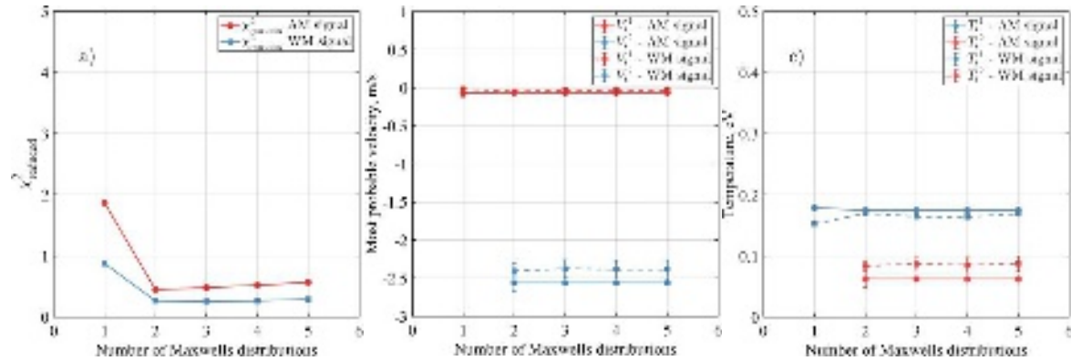
FIG. 10. a) \chi_{red}^2 evolution of fitting with number of Maxwellian distribution N ; b) most probable velocities of two main distributions; c) temperatures of two most probable distributions.
