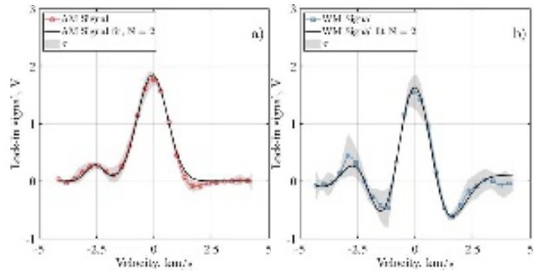
FIG. 12. The best fits of the a) AM signal and b) WM signal at the central location. N shows the number of Maxwellian distribution.
