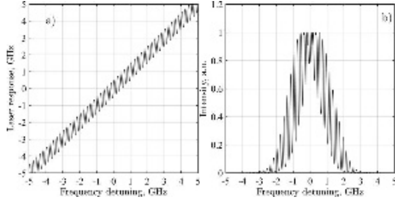
FIG. 15. (a) Laser response in WM configuration; (b) Simulated WM signal S(\nu, \nu_{WM}) , for a scan across of an absorption line.
