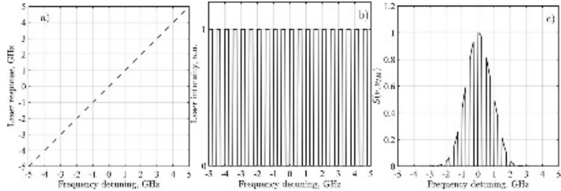
FIG. 14. a) laser frequency response and b) laser intensity response in intensity amplitude modulation configuration. Line interruptions represent zero amplitude of laser intensity. c) S(\nu, \nu_{AM}) function.
