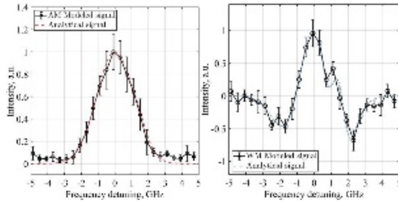
FIG. 4. (a) AM signal from the amplitude modulation model (black solid line) and its analytical form (red dashed line). (b) WM signal from the wavelength modulation model (black solid line) and its analytical form (blue dashed line).
