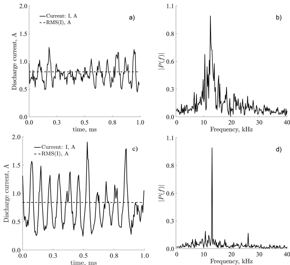
FIG. 1. Effect of the external drive on the discharge current: (a) discharge current trace without applied driving of the anode voltage, I_{\text{rms}}=0.81 \text{ A} ; (b) the corresponding FFT of the discharge current trace, f_{\max}=12.9 \text{ kHz} ; (c) discharge current trace with the anode voltage driving at 32 V peak-to-peak amplitude, I_{\text{rms}}=0.84 \text{ A} ; and (d) the corresponding FFT of the discharge current trace, f_{\max}=13.0 \text{ kHz} .
