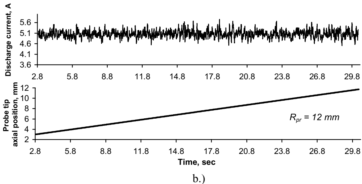
FIG. 2. Discharge current vs. time characteristics for V_d = 500 V and dm/dt = 50 SCCM.
