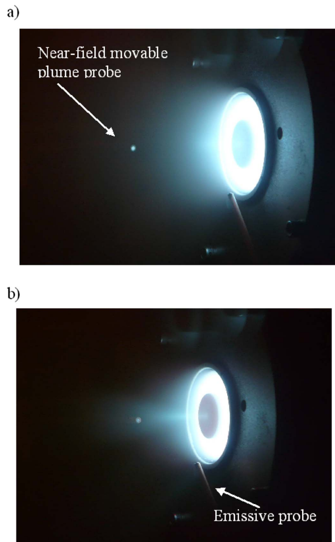
FIG. 6. (Color online) Plasma plume from the annular HT in the self-sustained and non-self-sustained regimes. The emissive probe is used to measure the plasma potential at the channel exit. A movable Langmuir probe is used to measure plasma properties in the near-field plume.
