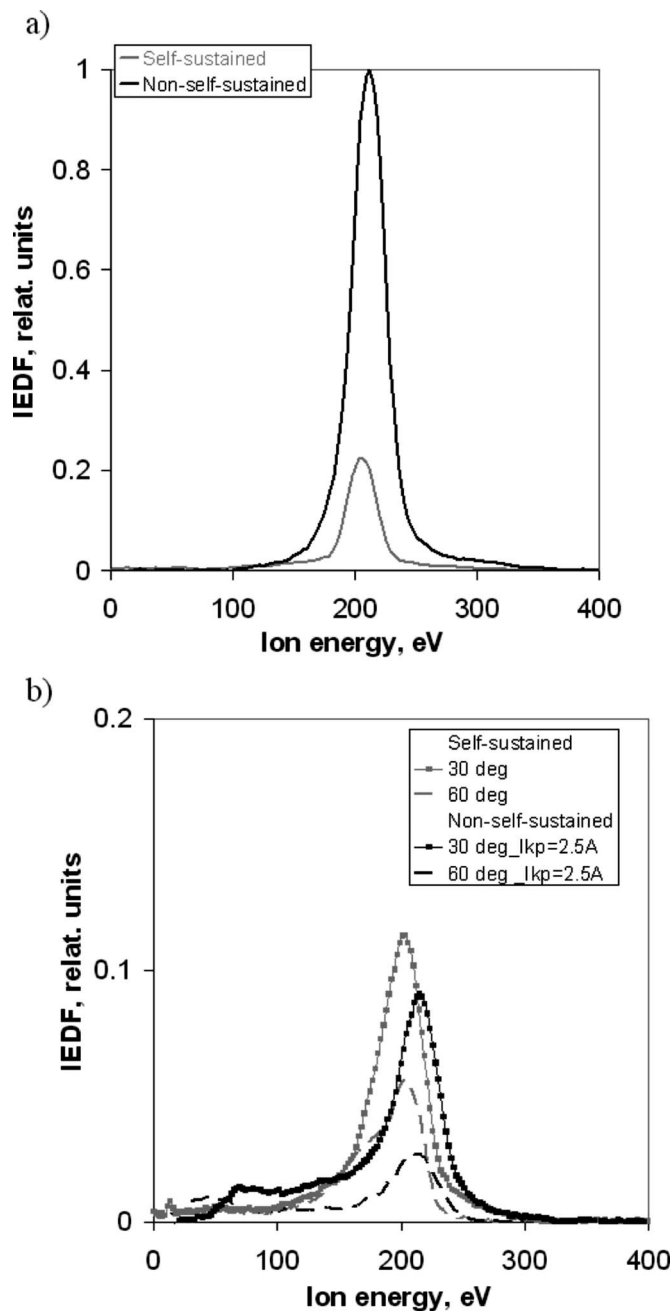
FIG. 7. Ion energy distribution function measured for the annular thruster in the far-field plume (70 cm from the thruster) at different angular positions of the retarding potential analyzer: (a) centerline and (b) 30° and 60° with the respect to the centerline. In both self-sustained and non-self-sustained regimes the thruster was operated with the same operating parameters (250 V and 3.4 SCCM) and the same magnetic field.
