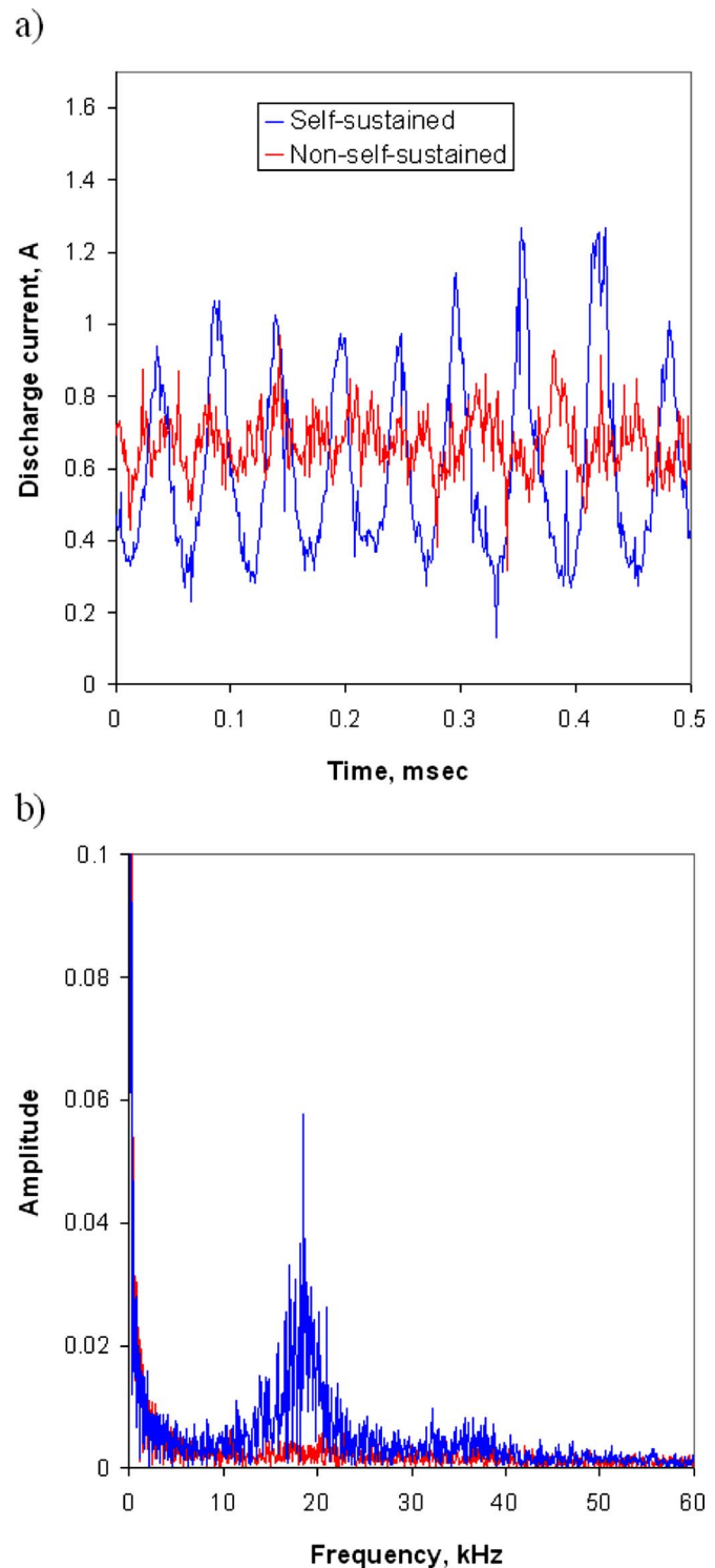
FIG. 10. (Color online) The oscilloscope traces of the discharge current oscillations (a) and corresponding frequency spectrum (b) for self-sustained and non-self-sustained regimes of the annular HT.
