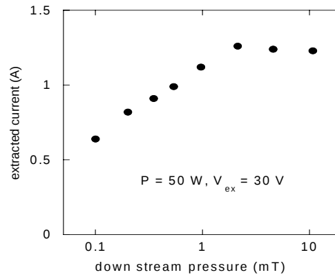
Figure 9. Extracted current versus downstream pressure.
