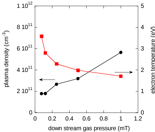
Figure 5. Plasma density and electron temperature versus downstream pressure.
