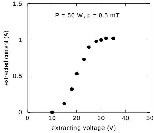
Figure 6. Extracted electron current versus extracting voltage.
