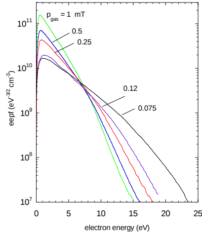
Figure 4. Electron energy probability functions for different downstream pressure, P = 100 W.
