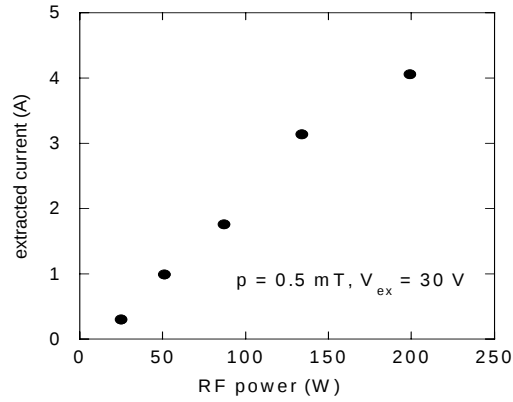
Figure 8. Extracted current versus RF power.
