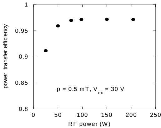
Figure 2. Power transfer efficiency versus RF power.
