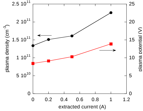
Figure 7. Plasma density and plasma potential versus extracted current.
