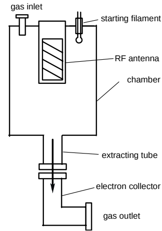
Figure 1. Schematic diagram of the plasma cathode.
