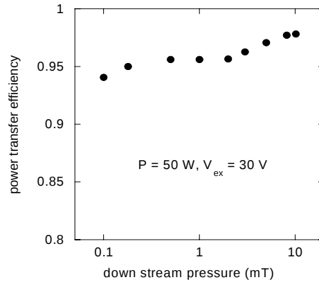
Figure 3. Power transfer efficiency versus downstream pressure.
