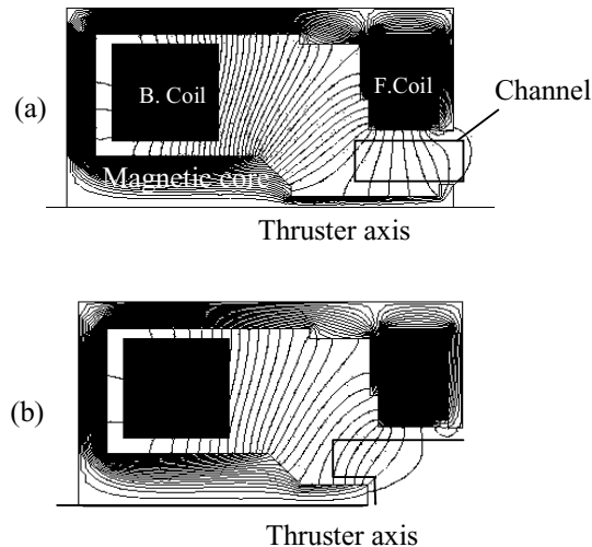
Fig. 2 Magnetic circuit of the annular thruster (a) and cylindrical (b) thruster. The channel OD diameter is 2.6 cm.
